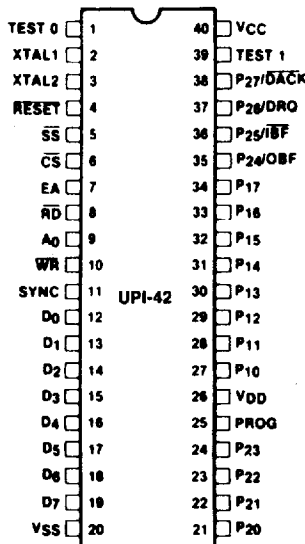
Figure 1. Pin Configuration
